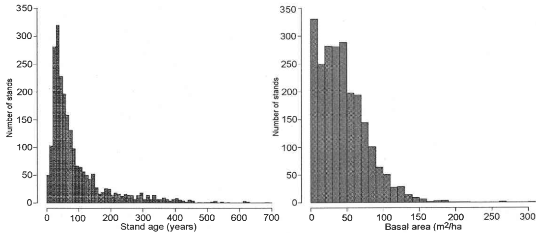
Fig. 2. Frequency distribution of sample polygons by stand age and basal area per ha.
