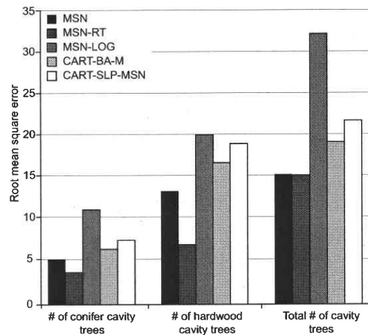
Fig. 3. Performance of imputation methods for estimating cavity tree abundance using 50% sampling intensity. MSN = Most Similar Neighbor; MSR-RT = Most Similar Neighbor with square root transformation; MSN-LOG = Most Similar Neighbor with logarithmic transformation; CART-BA-M = CART classified by basal area with MSN; CART-SLP-MSN = CART classified by slope with MSN.
