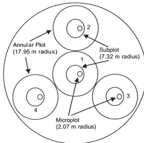
Forest Inventory and Analysis (FIA) plot design
